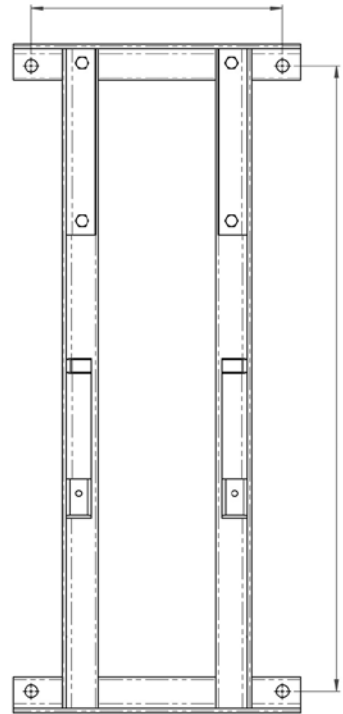
Figure 3: Hole pattern
