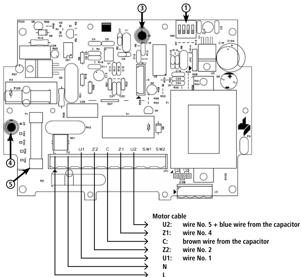
Figure 7: main control card diagram
